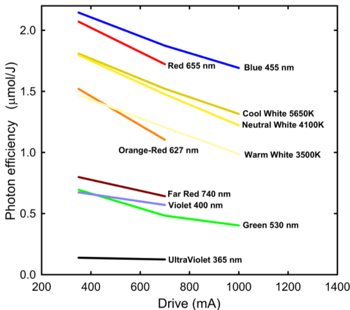
Figure 4. Effect of drive amperage and color on photon efficiency of LEDs. Data for Philips Lumileds LEDs (April 2013), courtesy of Mike Bourget, Orbitec.
