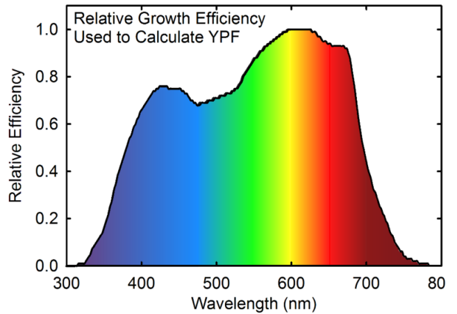
Figure 3. Yield photon flux curve. Effect of wavelength on relative photosynthesis per incident photon for a single leaf in low light [4].
