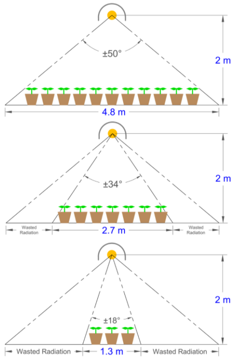
Figure 2 Canopy photon capture efficiency. As the plant growth area under the fixture gets smaller, wasted radiation often increases. Values are shown in meters, but this can be scaled as a unit-less ratio. Multiple overlapping fixtures are typically used to achieve uniform light distribution.
