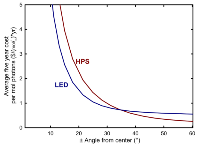
Figure 6. Effect of canopy capture efficiency on average five year cost. The cost per mole of photons for LEDs (Red/Blue LED from Lighting Sciences Group) becomes more favorable than the best HPS fixtures (Gavita) when the lighting area is less than \pm 35^\circ from center, assuming $0.11 per KWH cost of electricity and 3000 hours per year use.
