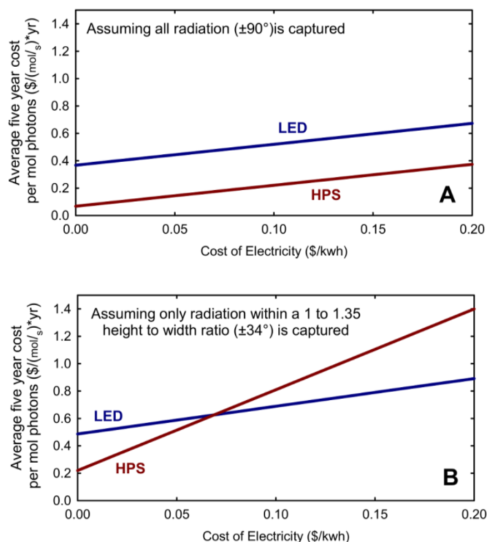
Figure 5. Effect of electricity cost on average five year cost for two capture assumptions. (A) When all radiation is assumed captured, HPS fixtures (Gavita) have a lower five-year cost per photon than LEDs (Red/Blue fixture, Lighting Sciences Group). (B) When only a narrow region below the fixture (±34°) is considered to be captured (e.g. on benches), the LEDs can have a lower cost per photon than HPS fixtures, but the cost per photon increases for both fixtures.
