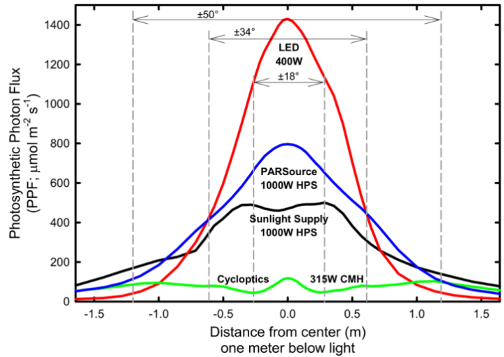
Figure 1 The light distribution of four fixtures with similar photon efficiency. The LED fixture (Lighting Sciences Group) uses optics to achieve a narrow distribution, with the majority of the photons falling in a concentrated pattern directly below the fixture. Conversely, the Cycloptics ceramic metal halide fixture is designed for even light distribution, and therefore casts uniform radiation over a large surface area. Since the area increases exponentially as the distance from the center increases, the photon flux farther from the center represents a larger quantity of total photons.
